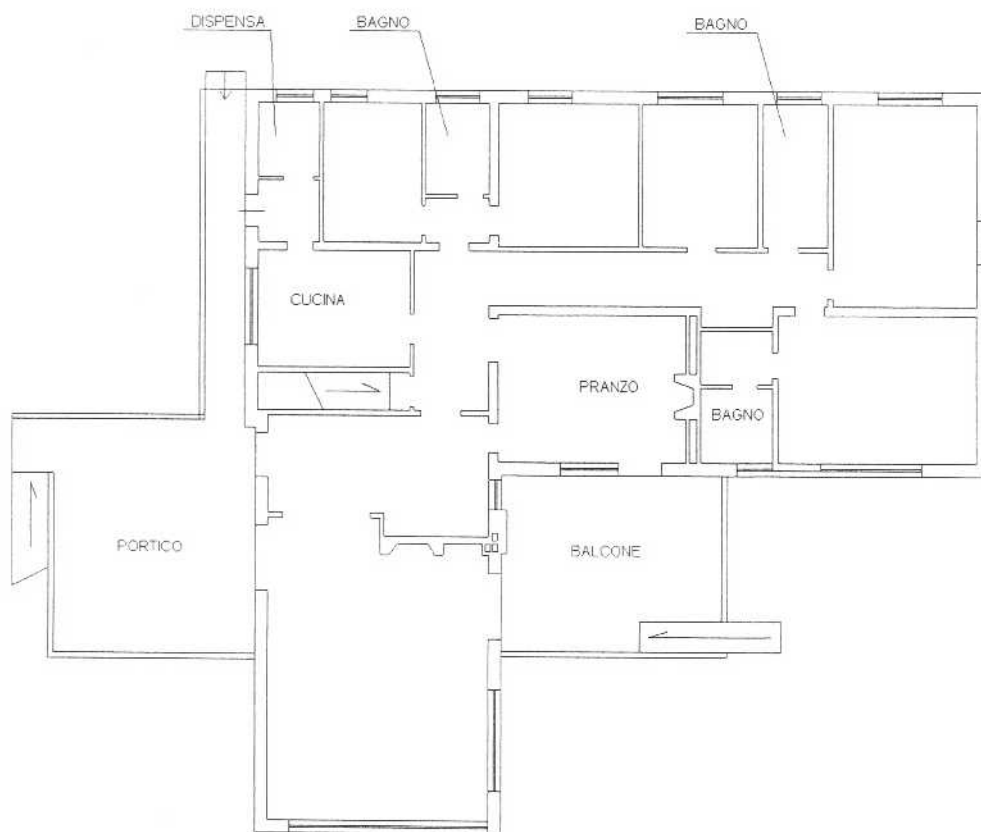
PIANTA PIANO SEMINTERRATO H=2,70ml
