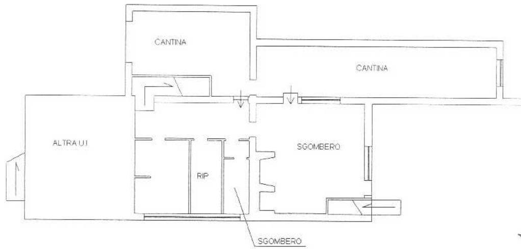
PIANTA PIANO SEMINTERRATO H=2,70ml
