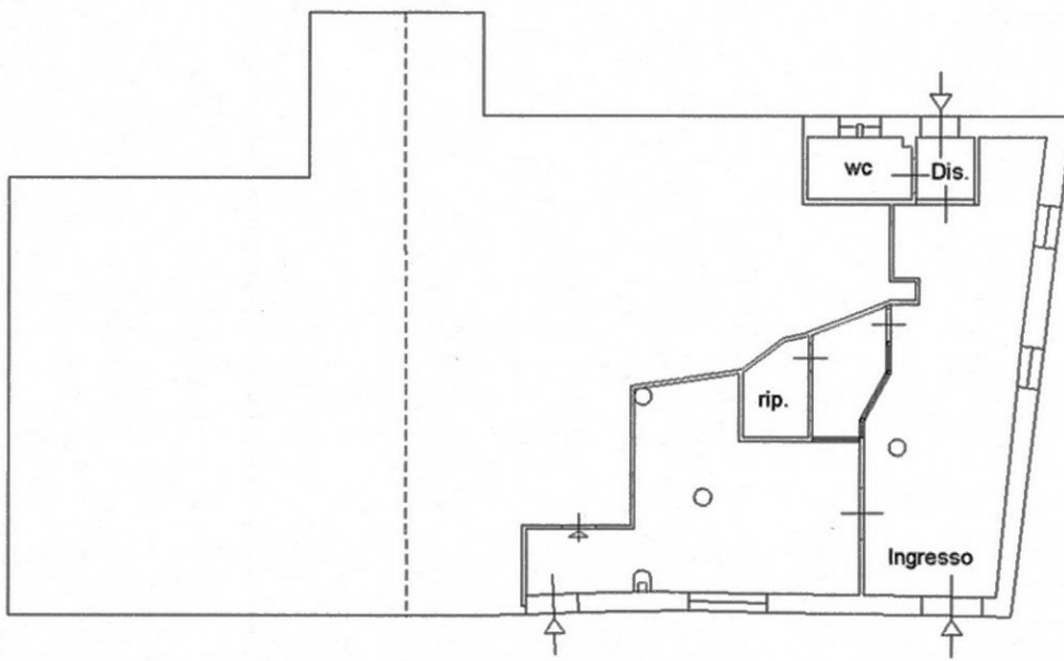
PIANO TERRA H=3,00
